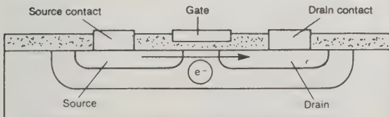
Typical horizontal transistor (insulating-gate field-effect transistor)
